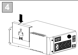
Align the battery compartment cover with the grooves in the UPS. Slide the cover down until it locks.
