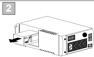
Pull the battery out, exposing the battery terminals and wires. Disconnect the wires from the terminals.
