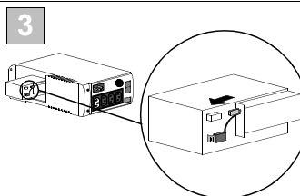
Slide the new battery into the battery compartment. Connect the battery wires to the terminals as follows: Black wire to Ground (-) terminal Red wire to Positive (+) terminal
